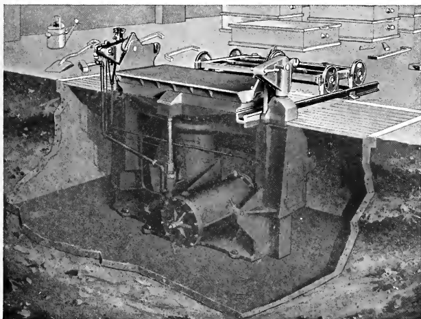
Fig. 148. A 64-inch Roll-Over Jolt-Moulding Machine, showing Section through Foundation.
